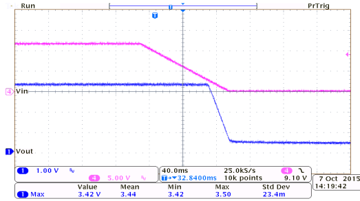
Power Off Response: HT75E33 ( I_{OUT}=0mA , T_{FALL}=100ms )
