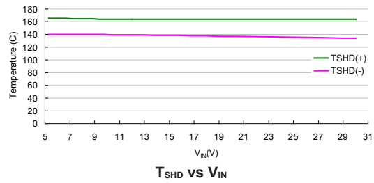
T_{SHD} vs V_{IN}
