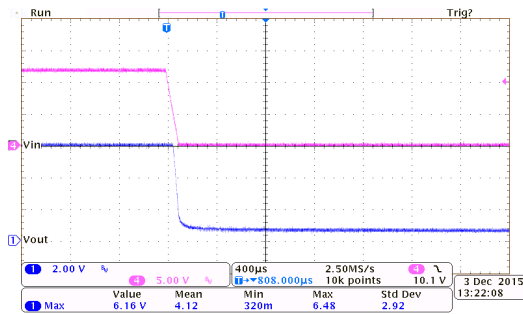
Power Off Response: HT75E60 ( I_{OUT}=0mA , T_{FALL}=0.1ms )
