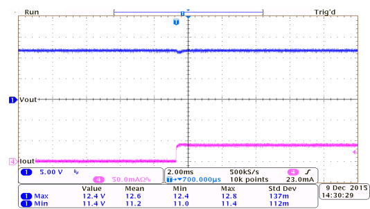
Load Transient Response: HT75E60 ( V_{IN}=8.0V , I_{OUT}=40mA to 0mA )
