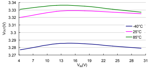
Line Regulation: HT75E33 ( I_{OUT}=10mA )
