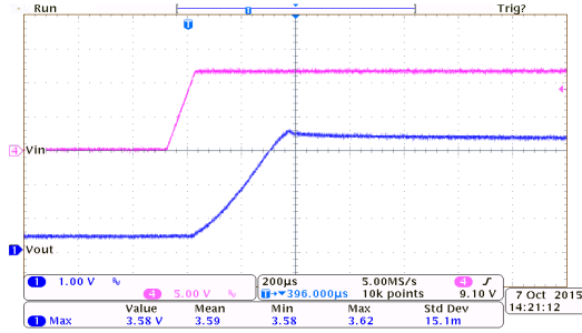
Power On Response: HT75E33 ( I_{OUT}=0mA , T_{RISE}=0.1ms )
