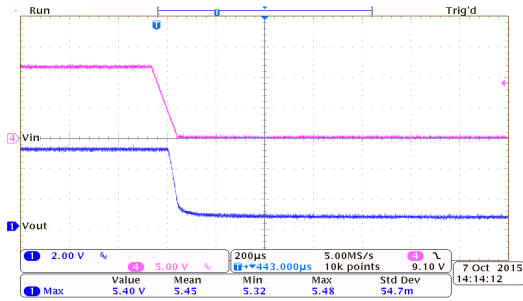
Power Off Response: HT75E50 ( I_{OUT}=0mA , T_{FALL}=0.1ms )
