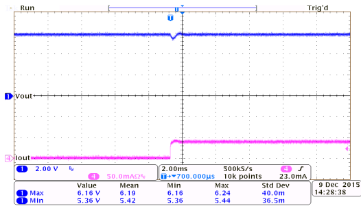
Load Transient Response: HT75E60 ( V_{IN}=8.0V , I_{OUT}=0mA to 40mA )
