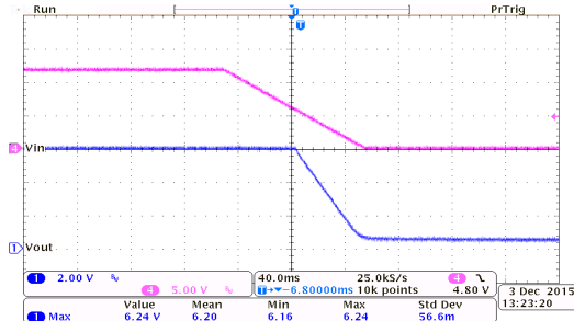
Power Off Response: HT75E60 ( I_{OUT}=0mA , T_{FALL}=100ms )
