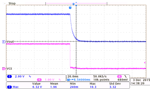
ON/OFF Response: HT75E60 ( I_{OUT}=150mA , V_{CE}=2.7V to 0V)
