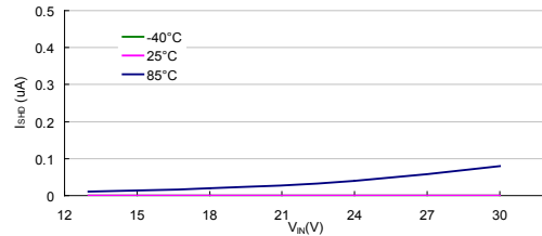
I SHD vs V IN : HT75E60 (I OUT =0mA)
