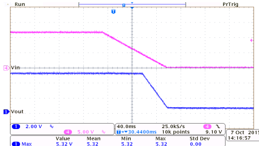
Power Off Response: HT75E50 ( I_{OUT}=0mA , T_{FALL}=100ms )
