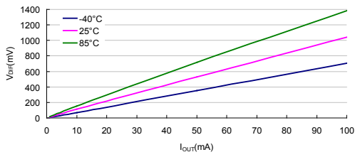
Dropout voltage: HT75E33
