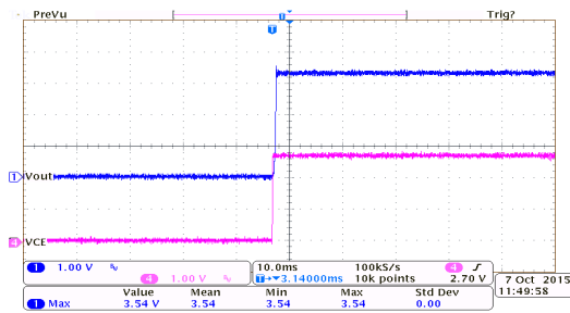
ON/OFF Response: HT75E33 ( I_{OUT}=100mA , V_{CE}=0V to 2.7V)
