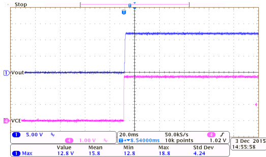
ON/OFF Response: HT75EC0 ( I_{OUT}=150mA , V_{CE}=0V to 2.7V)
