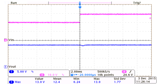
Line Transient Response: HT75EC0 ( I_{OUT}=10mA )
