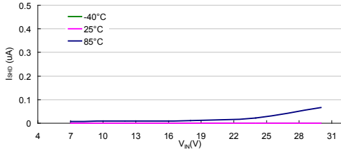
I SHD vs V IN : HT75E60 (I OUT =0mA)
