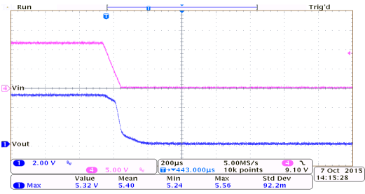
Power Off Response: HT75E50 ( I_{OUT}=150mA , T_{FALL}=0.1ms )
