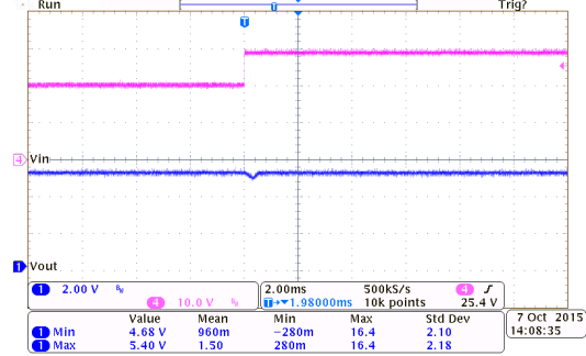
Line Transient Response: HT75E50 ( I_{OUT}=10mA )
