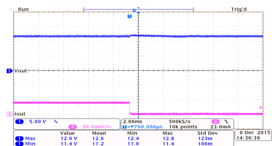
Load Transient Response: HT75EC0 ( V_{IN}=14V , I_{OUT}=40mA to 0mA )
