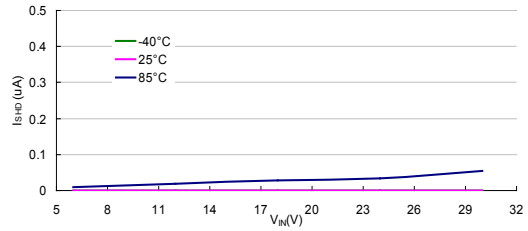
I SHD vs V IN : HT75E33 (I OUT =0mA)
