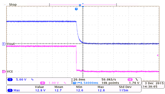
ON/OFF Response: HT75EC0 ( I_{OUT}=0mA , V_{CE}=2.7V to 0V)
