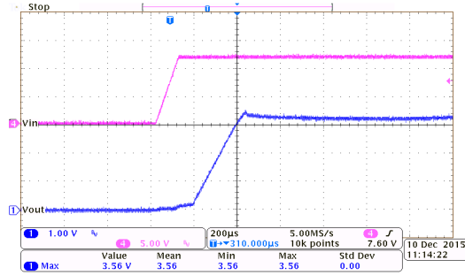
Power On Response: HT75E33 ( I_{OUT}=100mA , T_{RISE}=0.1ms )
