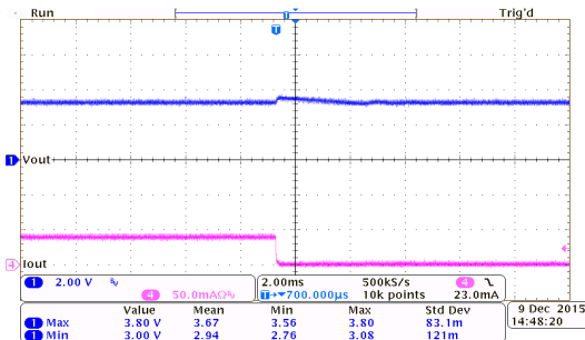
Load Transient Response: HT75E33 ( V_{IN}=5.3V , I_{OUT}=40mA to 0mA )
