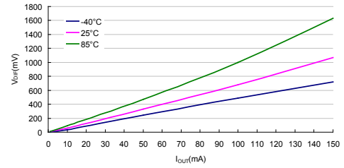
Dropout voltage: HT75EC0
