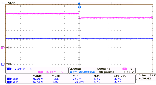
Line Transient Response: HT75E60 ( I_{OUT}=10mA )
