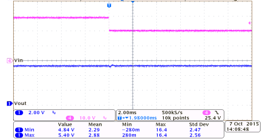
Line Transient Response: HT75E50 ( I_{OUT}=10mA )
