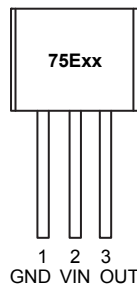
TO92-3
