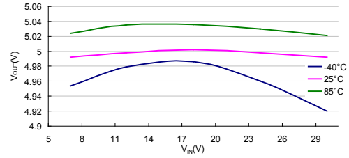
Line Regulation: HT75E50 ( I_{OUT}=10mA )
