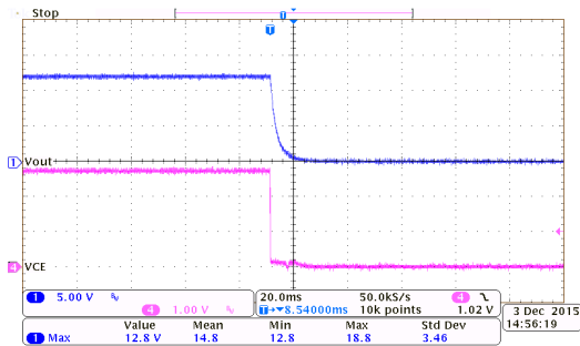
ON/OFF Response: HT75EC0 ( I_{OUT}=150mA , V_{CE}=2.7V to 0V)
