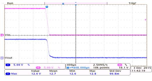
Power Off Response: HT75EC0 ( I_{OUT}=150mA , T_{FALL}=0.1ms )
