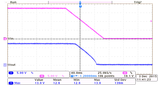
Power Off Response: HT75EC0 ( I_{OUT}=150mA , T_{FALL}=100ms )
