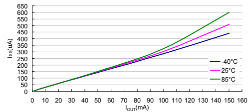
I SS vs I OUT : HT75E60 (V IN =14V)
