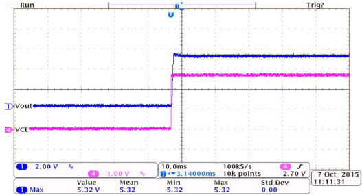
ON/OFF Response: HT75E50 ( I_{OUT}=0mA , V_{CE}=0V to 2.7V)
