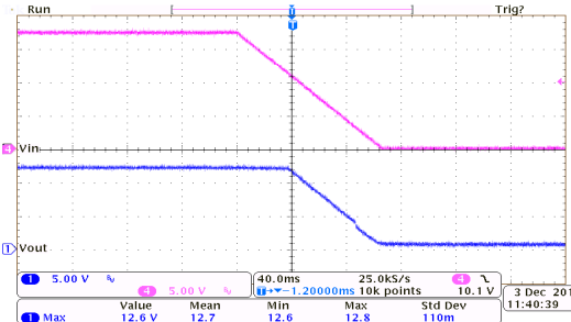
Power Off Response: HT75EC0 ( I_{OUT}=0mA , T_{FALL}=100ms )
