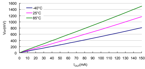
Dropout voltage: HT75E60
