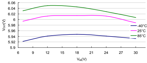
Line Regulation: HT75E60 ( I_{OUT}=10mA )
