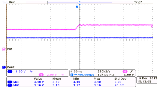
Line Transient Response: HT75E33 ( I_{OUT}=10mA )
