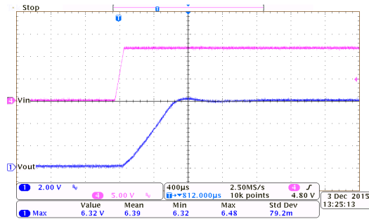
Power On Response: HT75E60 ( I_{OUT}=150mA , T_{RISE}=0.1ms )
