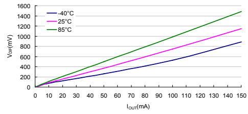
Dropout voltage: HT75E50
