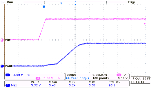
Power On Response: HT75E50 ( I_{OUT}=150mA , T_{RISE}=0.1ms )
