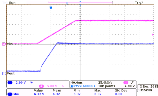
Power On Response: HT75E60 ( I_{OUT}=150mA , T_{RISE}=100ms )
