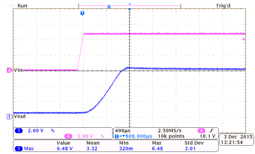
Power On Response: HT75E60 ( I_{OUT}=0mA , T_{RISE}=0.1ms )
