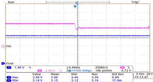
Line Transient Response: HT75E33 ( I_{OUT}=10mA )
