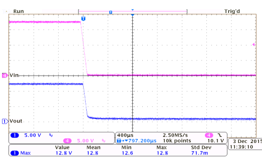
Power Off Response: HT75EC0 ( I_{OUT}=0mA , T_{FALL}=0.1ms )
