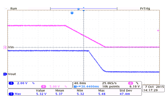
Power Off Response: HT75E50 ( I_{OUT}=150mA , T_{FALL}=100ms )
