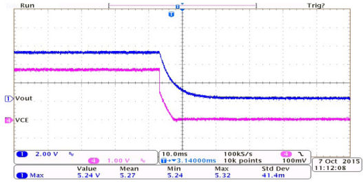
ON/OFF Response: HT75E50 ( I_{OUT}=0mA , V_{CE}=2.7V to 0V)
