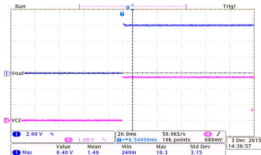
ON/OFF Response: HT75E60 ( I_{OUT}=0mA , V_{CE}=0V to 2.7V)
