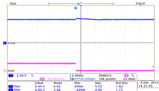
Load Transient Response: HT75E50 ( V_{IN}=7.0V , I_{OUT}=40mA to 0mA )
