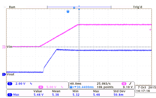
Power On Response: HT75E50 ( I_{OUT}=150mA , T_{RISE}=100ms )
