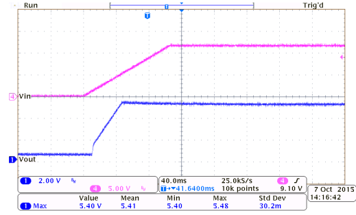
Power On Response: HT75E50 ( I_{OUT}=0mA , T_{RISE}=100ms )
