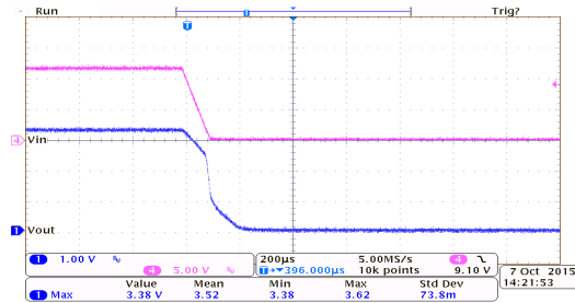
Power Off Response: HT75E33 ( I_{OUT}=100mA , T_{FALL}=0.1ms )
