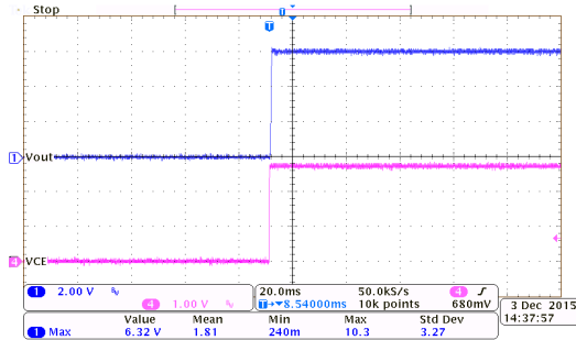
ON/OFF Response: HT75E60 ( I_{OUT}=150mA , V_{CE}=0V to 2.7V)
