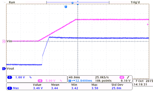
Power On Response: HT75E33 ( I_{OUT}=0mA , T_{RISE}=100ms )
