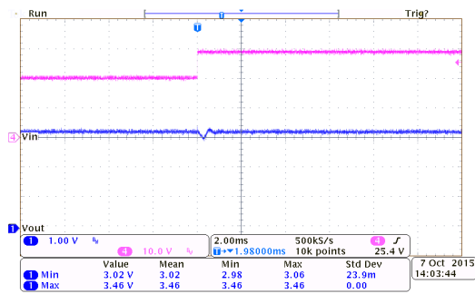
Line Transient Response: HT75E33 ( I_{OUT}=10mA )
