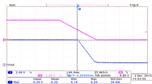
Power Off Response: HT75E60 ( I_{OUT}=150mA , T_{FALL}=100ms )
