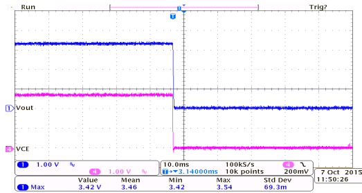
ON/OFF Response: HT75E33 ( I_{OUT}=100mA , V_{CE}=2.7V to 0V)
