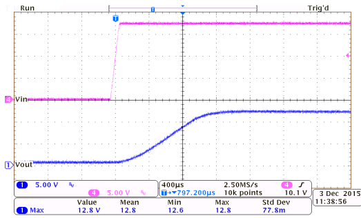
Power On Response: HT75EC0 ( I_{OUT}=0mA , T_{RISE}=0.1ms )
