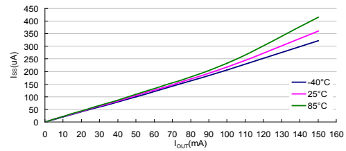
I SS vs I OUT : HT75E50 (V IN =7.0V)
