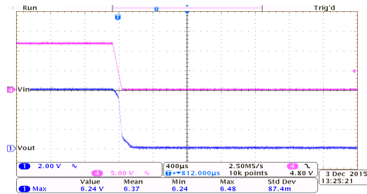
Power Off Response: HT75E60 ( I_{OUT}=150mA , T_{FALL}=0.1ms )
