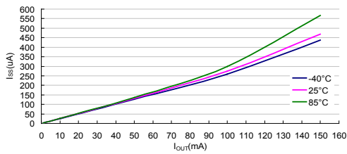
I SS vs I OUT : HT75E60 (V IN =8.0V)
