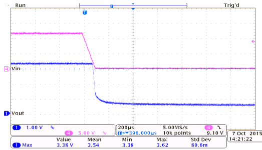
Power Off Response: HT75E33 ( I_{OUT}=0mA , T_{FALL}=0.1ms )
