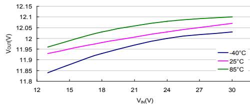
Line Regulation: HT75EC0 ( I_{OUT}=10mA )
