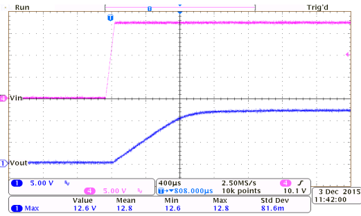
Power On Response: HT75EC0 ( I_{OUT}=150mA , T_{RISE}=0.1ms )
