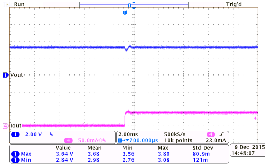
Load Transient Response: HT75E33 ( V_{IN}=5.3V , I_{OUT}=0mA to 40mA )
