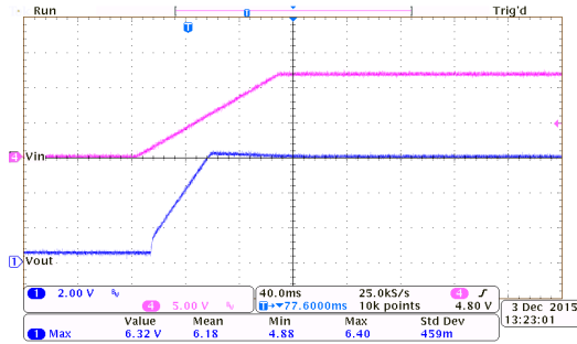
Power On Response: HT75E60 ( I_{OUT}=0mA , T_{RISE}=100ms )
