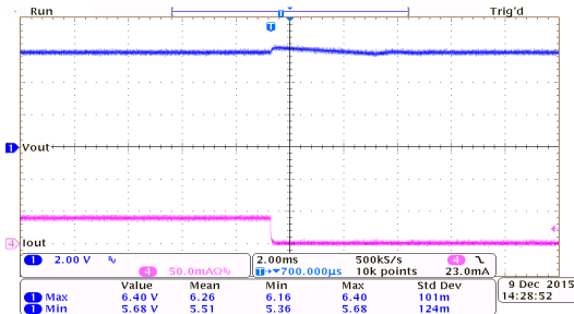
Load Transient Response: HT75E60 ( V_{IN}=8.0V , I_{OUT}=40mA to 0mA )
