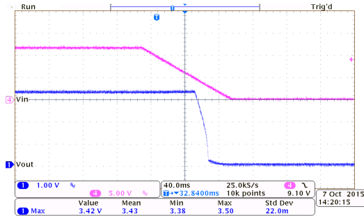
Power Off Response: HT75E33 ( I_{OUT}=100mA , T_{FALL}=100ms )
