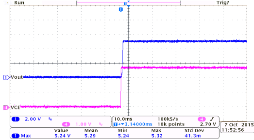
ON/OFF Response: HT75E50 ( I_{OUT}=150mA , V_{CE}=0V to 2.7V)
