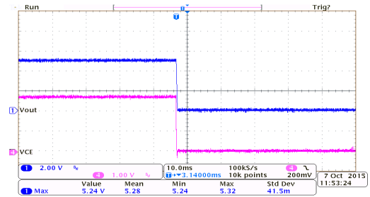
ON/OFF Response: HT75E50 ( I_{OUT}=150mA , V_{CE}=2.7V to 0V)
