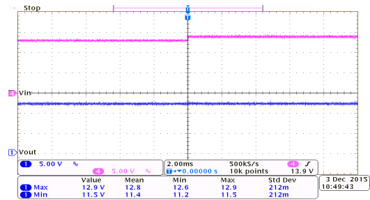
Line Transient Response: HT75EC0 ( I_{OUT}=10mA )
