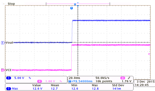
ON/OFF Response: HT75E60 ( I_{OUT}=0mA , V_{CE}=2.7V to 0V)
