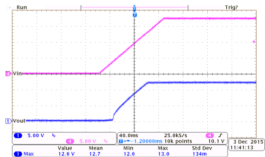
Power On Response: HT75EC0 ( I_{OUT}=150mA , T_{RISE}=100ms )
