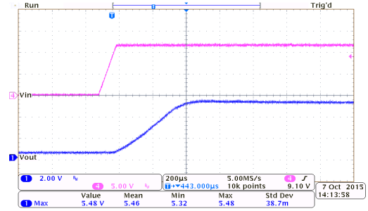
Power On Response: HT75E50 ( I_{OUT}=0mA , T_{RISE}=0.1ms )
