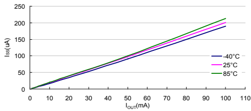
I SS vs I OUT : HT75E33 (V IN =5.3V)
