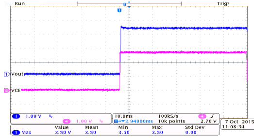
ON/OFF Response: HT75E33 ( I_{OUT}=0mA , V_{CE}=0V to 2.7V)
