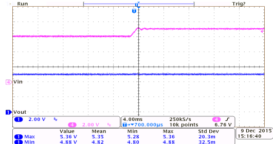
Line Transient Response: HT75E50 ( I_{OUT}=10mA )
