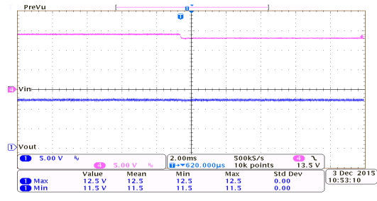
Line Transient Response: HT75EC0 ( I_{OUT}=10mA )
