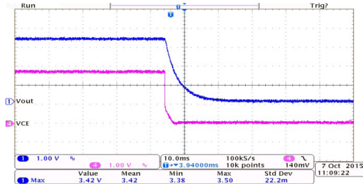
ON/OFF Response: HT75E33 ( I_{OUT}=0mA , V_{CE}=2.7V to 0V)
