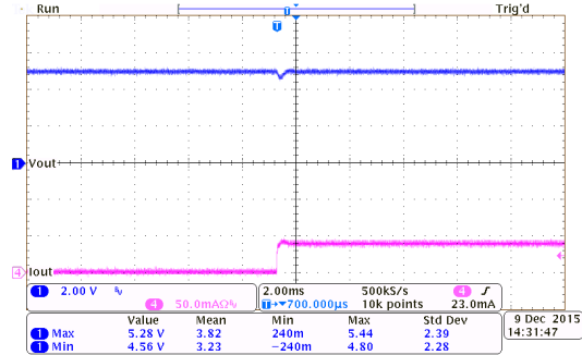
Load Transient Response: HT75E50 ( V_{IN}=7V , I_{OUT}=0mA to 40mA )
