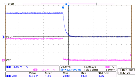
ON/OFF Response: HT75E60 ( I_{OUT}=0mA , V_{CE}=2.7V to 0V)
