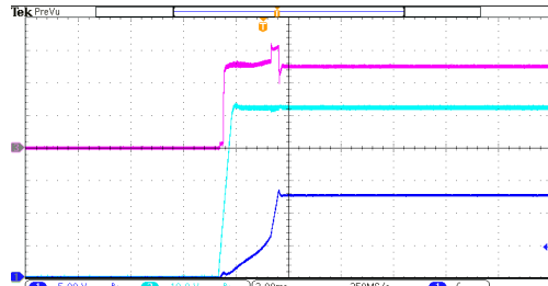
Power Up (HT7463C, V_{IN}=52V , I_{OUT}=500mA )
