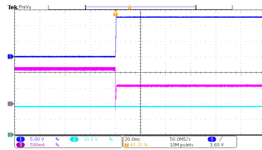
Short Recovery (HT7463D, I_{OUT}=500mA )
