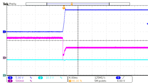
Short Recovery (HT7463C, I_{OUT}=500mA )
