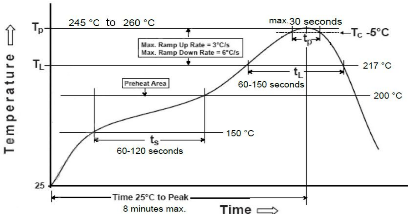
Figure 7: SSW292B Typical Lead-free Soldering Profile
