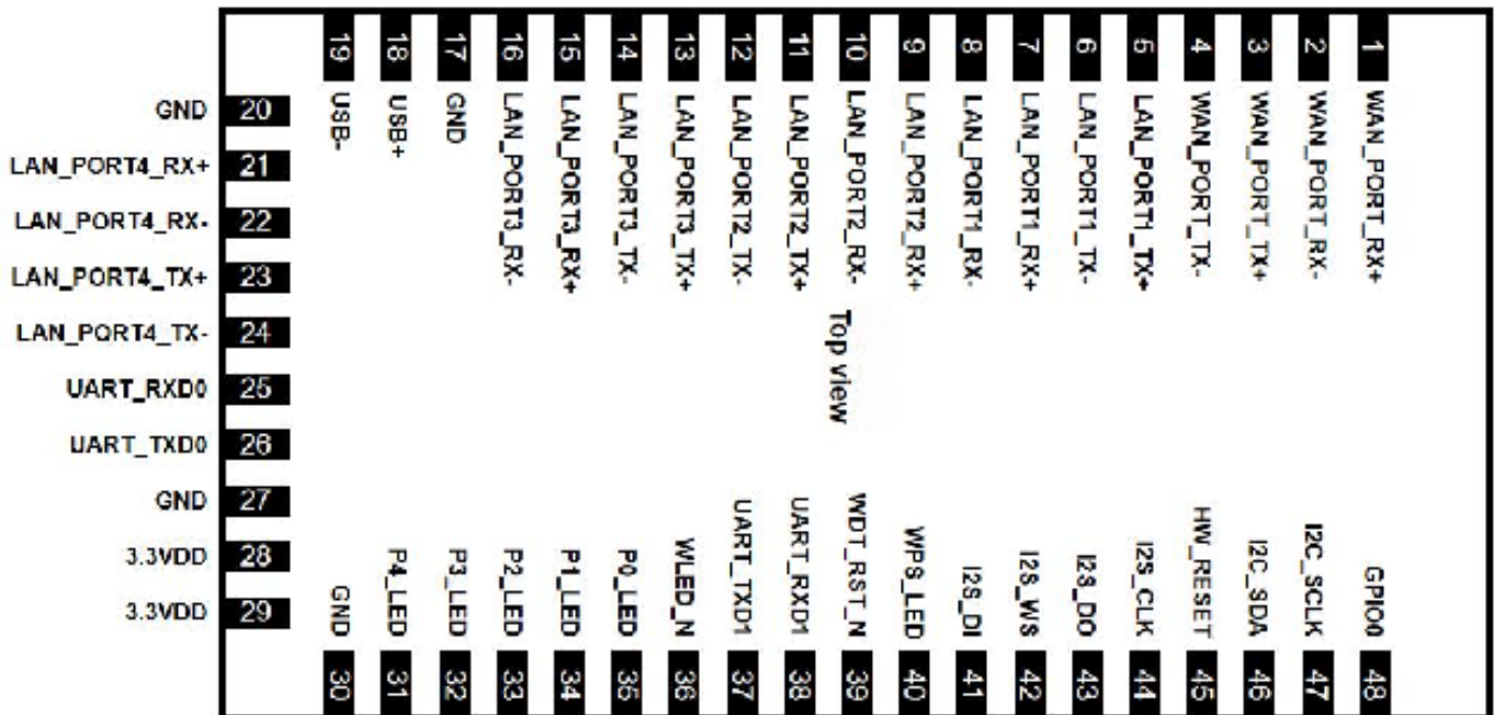
Figure 5: SSW292B Pin Package
