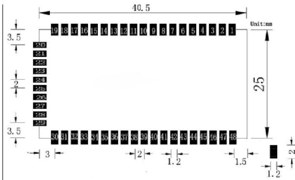
Figure 6: SSW292B Recommend PCB Footprint
