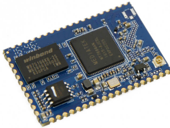
Figure 1: SSW292B Top View
