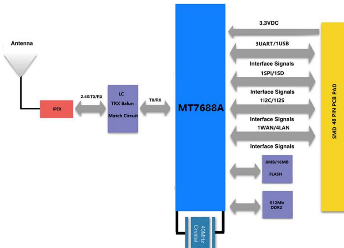
Figure 2: SSW292B Block Diagram
